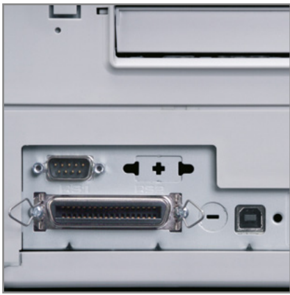
RS 232, IEEE 1284 AND USB 2.0 INTERFACES additional options: second USB port, second serial port, LAN interface
